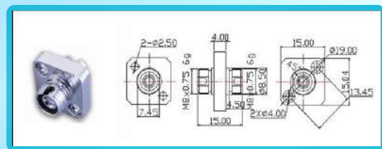
Fig 4. FC D Adapter
