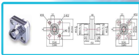
Fig 1. FC Square Solid Body Adapter
