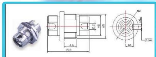
Fig 2. FC Square Twain Adapter
