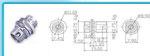
Fig 5. FC D3 Adapter
