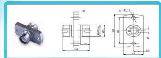
Fig 3. FC Rectangle Adapter
