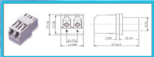
Fig 3. LC SC Footprint Duplex Adapter
