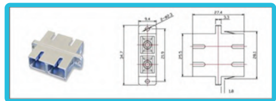
Fig 4. LC SC Footprint Quad Adapter
